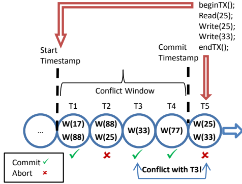
Figure 4: Conflict detection under snapshot isolation: a transaction commits if no other committed transaction in its conflict window has an overlapping write-set.
