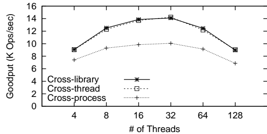
Figure 8: YCSB over different compositions of IsoBT and IsoHT.
